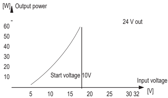
Figure 6. Output power PM80 24/24-24
