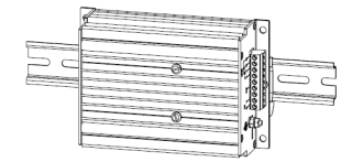
PM50/80 Wall or DIN-rail mounted (standard)
