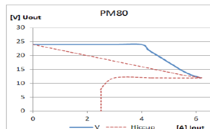
Figure 4. Current limit characteristic for PM80*/24-24 with outputs connected in parallel.
