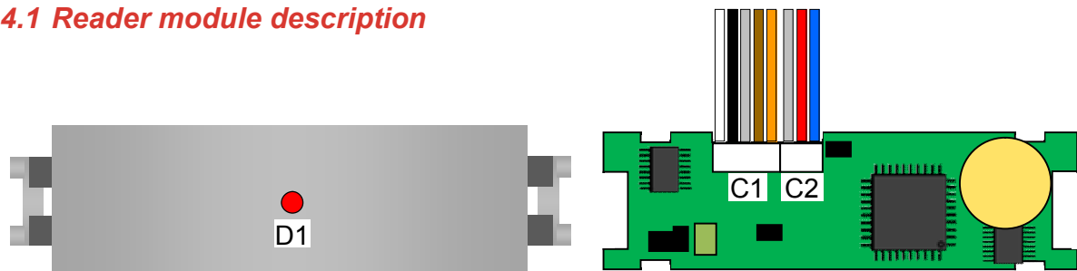
Pic. 2: MREM 80 reader module, front (left) and rear (right) view
