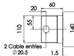
TITAN COMPACT (Recessed version)
