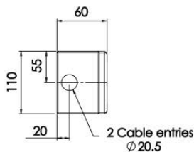
TITAN COMPACT (Wall mounting version)
