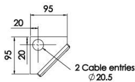
TITAN COMPACT A45
